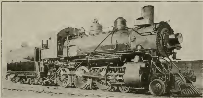
NO. 26, SAN DIEGO & ARIZONA RAILWAY CHANGED FROM SATURATED SLIDE VALVE INSIDE STEAM PIPE TO SUPERHEATED PISTON VALVE OUTSIDE STEAM PIPE LOCOMOTIVE
